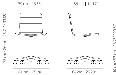
KLBRB lines upholstery
