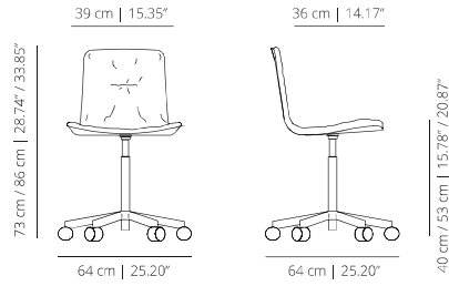
KLBR soft upholstery
