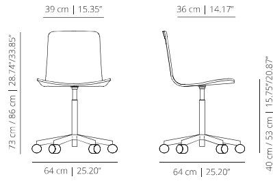
KLBR smooth upholstery
