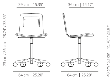
KLBRROCR | KLBR_CR stained with cushion | lacquered with cushion
